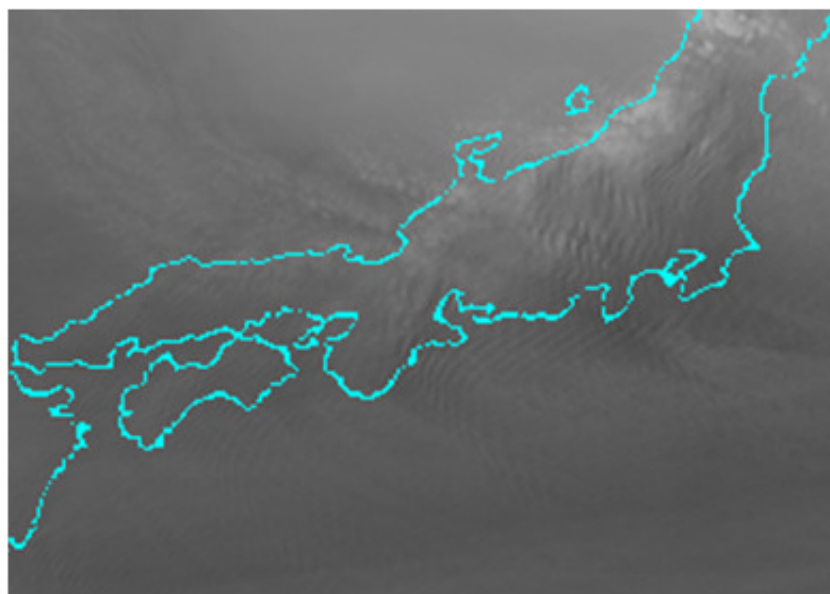
Himawari-8 channel 9 (6.9 microns), 0240UTC 18 December 2014
