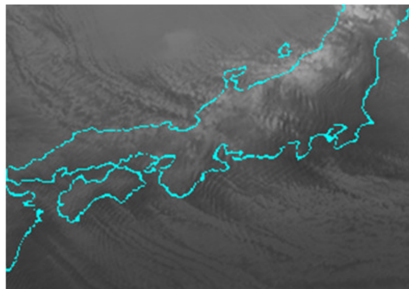
Himawari-8 channel 10 (7.3 microns), 0240UTC 18 December 2014
