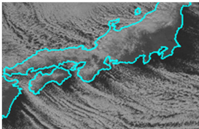
MTSAT-2, channel 1, 0232UTC 18 December 2014
